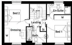
First Floor Plan 1:100
