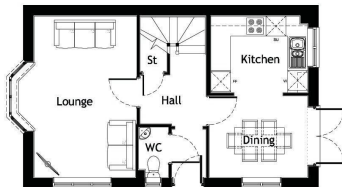
Ground Floor Plan 1:100
