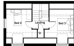
Second Floor Plan 1:100
