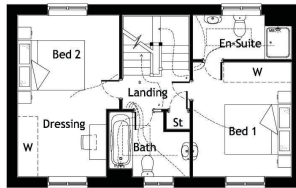
First Floor Plan 1:100
